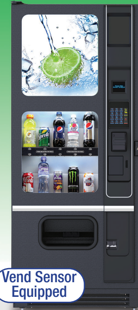
VendRevv BC10 Bottle & Can Vendor 72" x 31.75"W x 36.125"D *Ship Weight 671 lbs, 10 selections Capacity: 500-12oz cans / 240-20 oz bottles or combination of cans and bottles Standard vend sizes in ounces: 12, 16.9, 20 & 24 Optional kit needed for 250ml Energy Drink cans.
